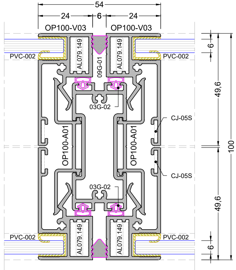
DETAY - 2 DETAIL - 2
