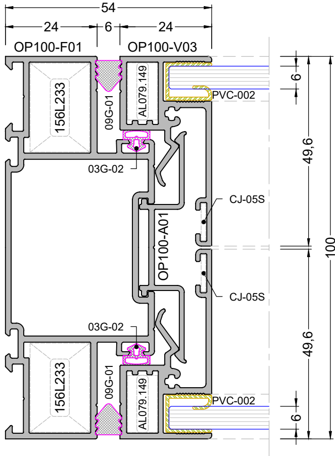
DETAY - 1 DETAIL - 1
