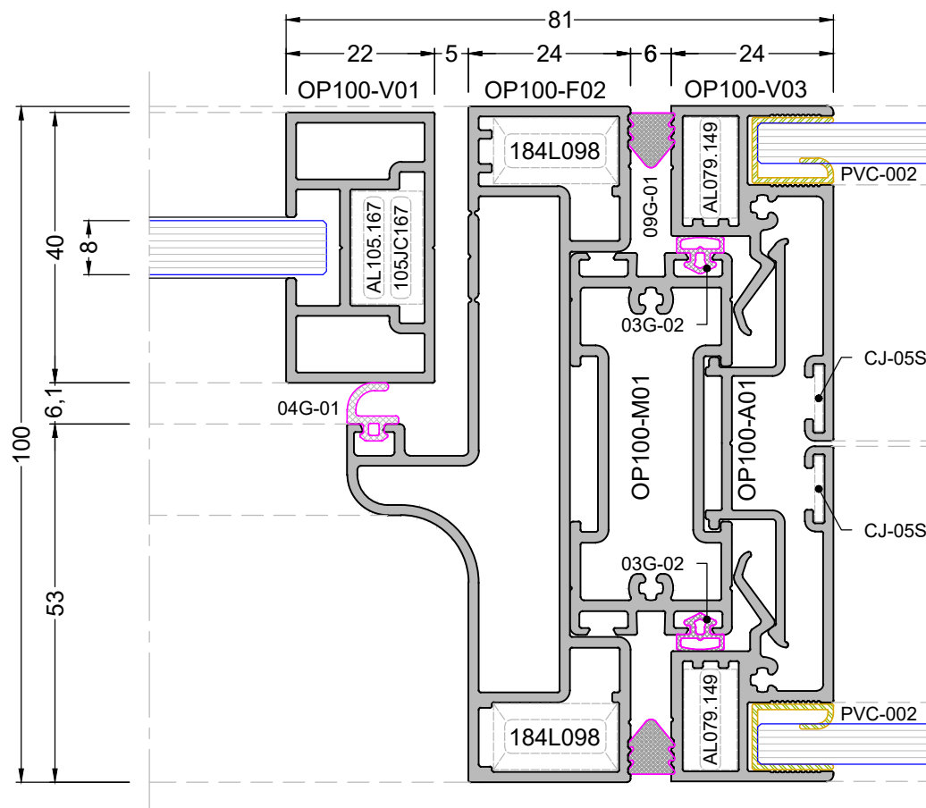
DETAY - 4 DETAIL - 4
