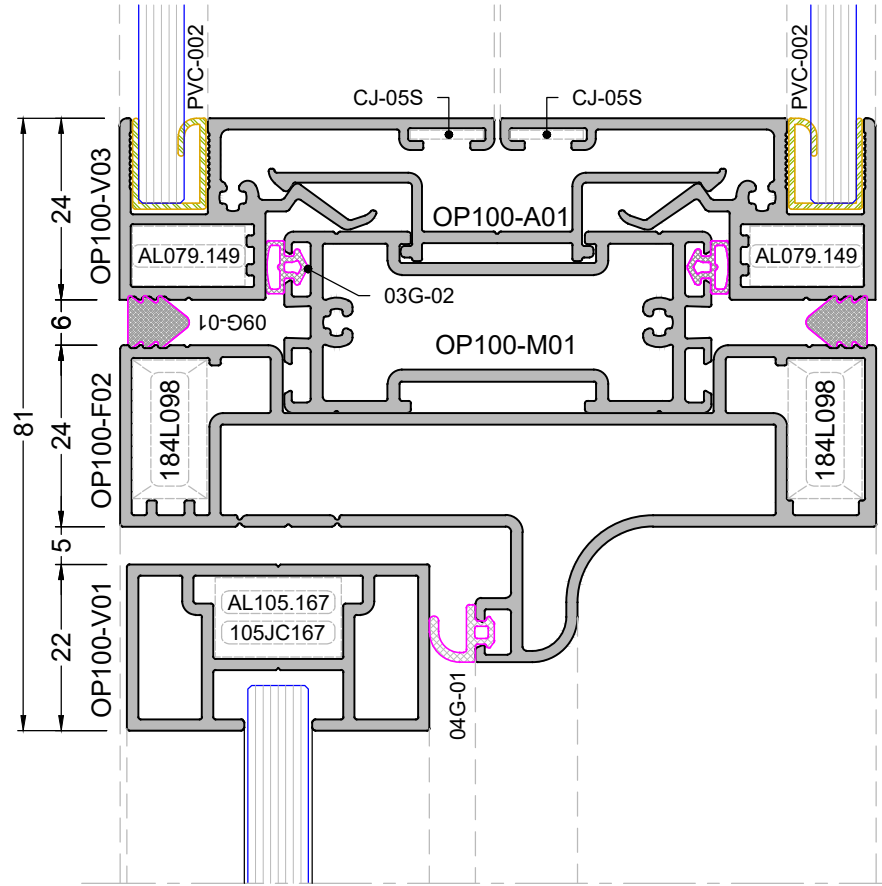
DETAY -12 DETAIL - 12
