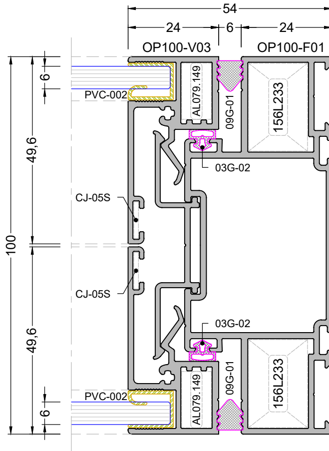
DETAY - 7 DETAIL - 7
