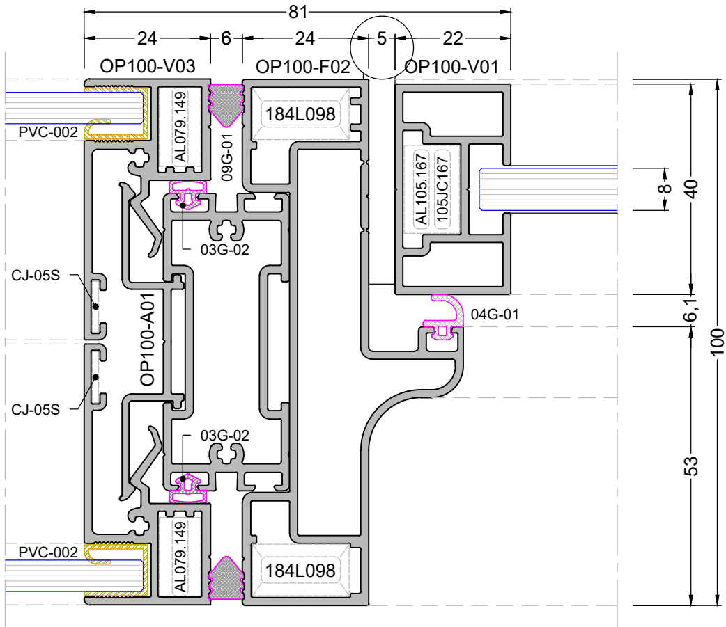
DETAY - 3 DETAIL - 3
