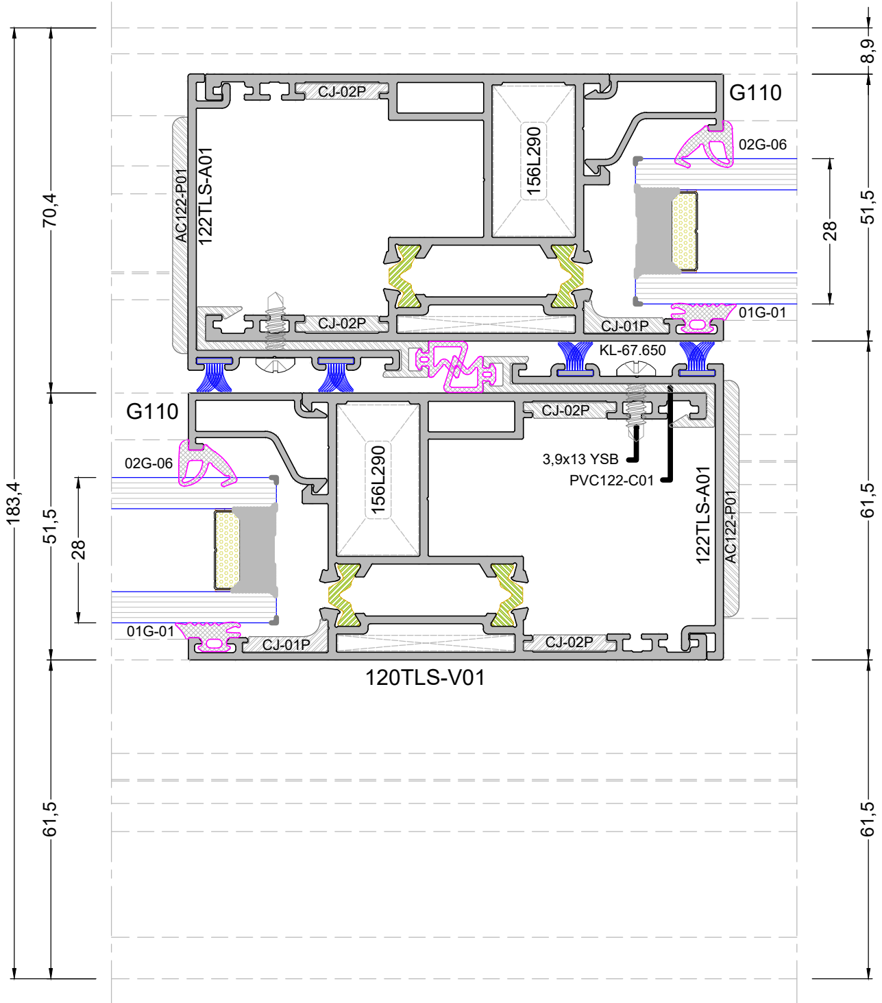
DETAY 3-3 DETAIL 3-3
