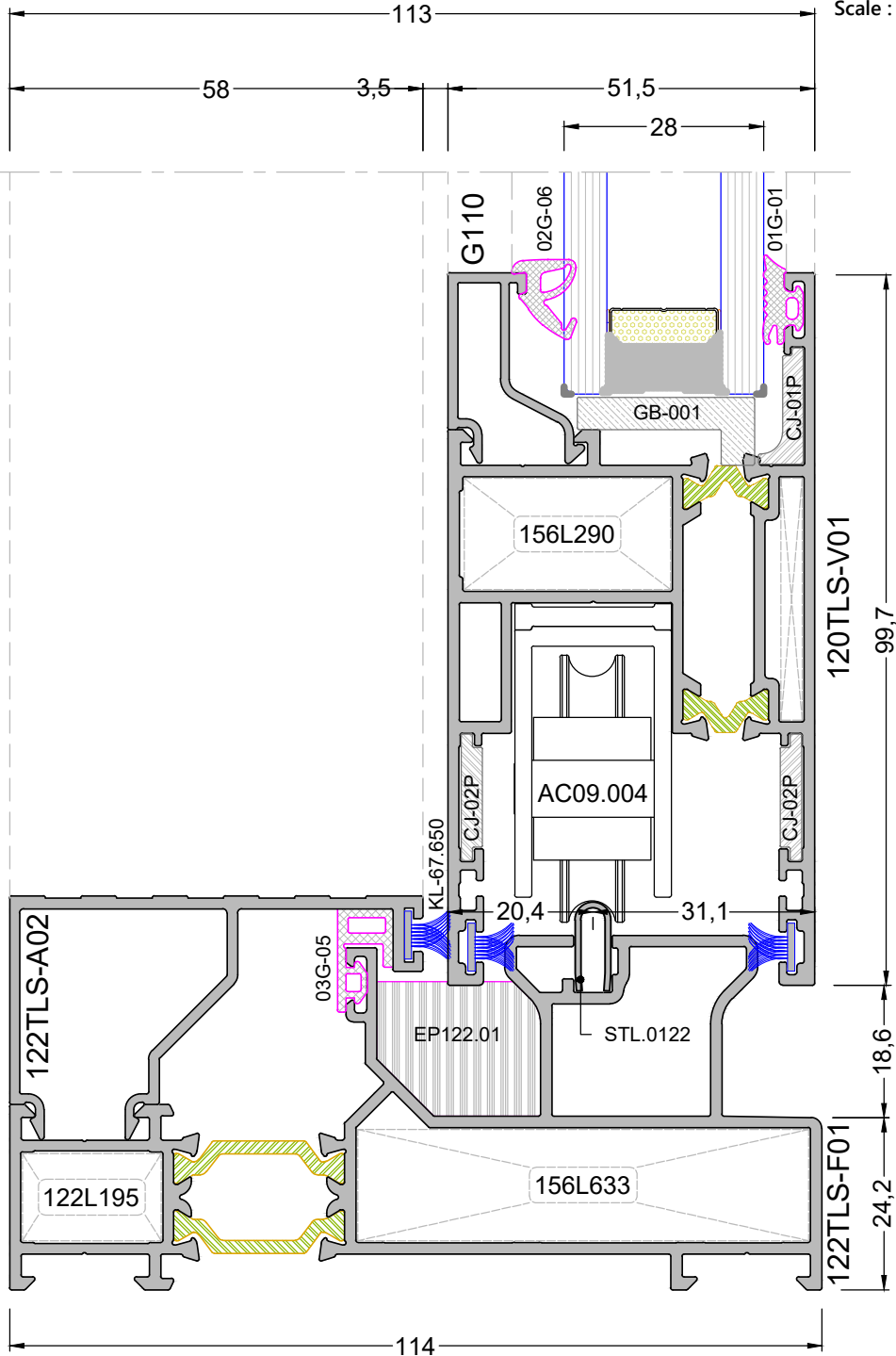
DETAY 1-18 DETAIL 1-18
