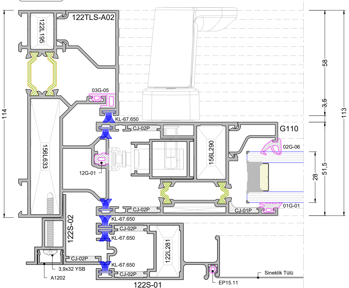
DETAY 1-24 DETAIL 1-24
