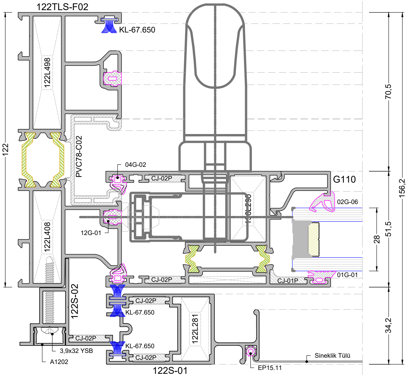
DETAY 2-9 DETAIL 2-9
