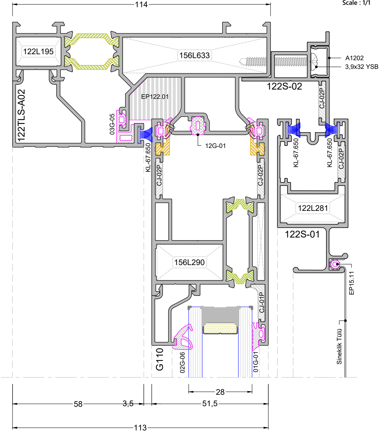
DETAY 1-14 DETAIL 1-14
