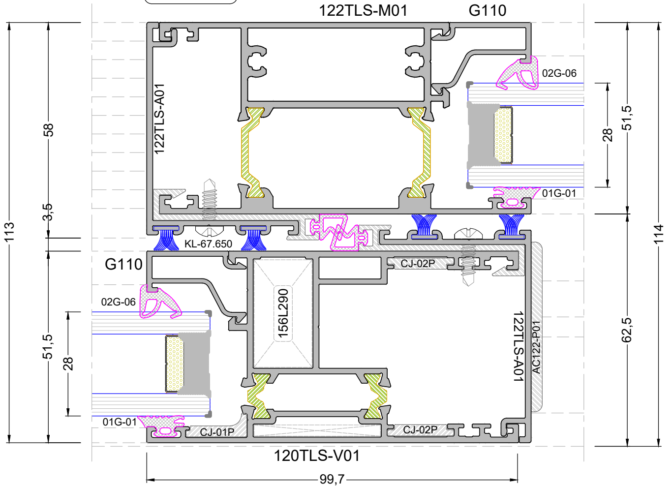
DETAY 1-2 DETAIL 1-2
