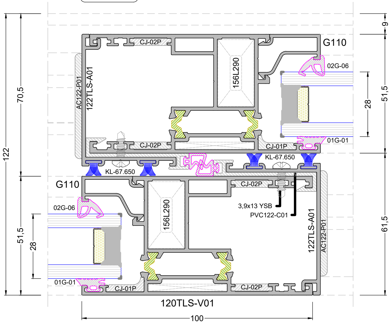
DETAY 2-15 DETAIL 2-15
