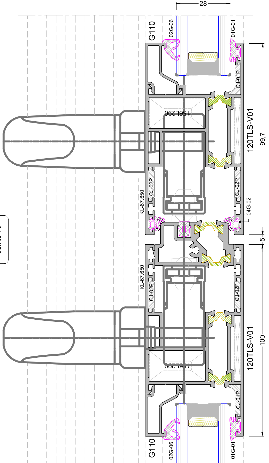
DETAY 1-9 DETAIL 1-9
