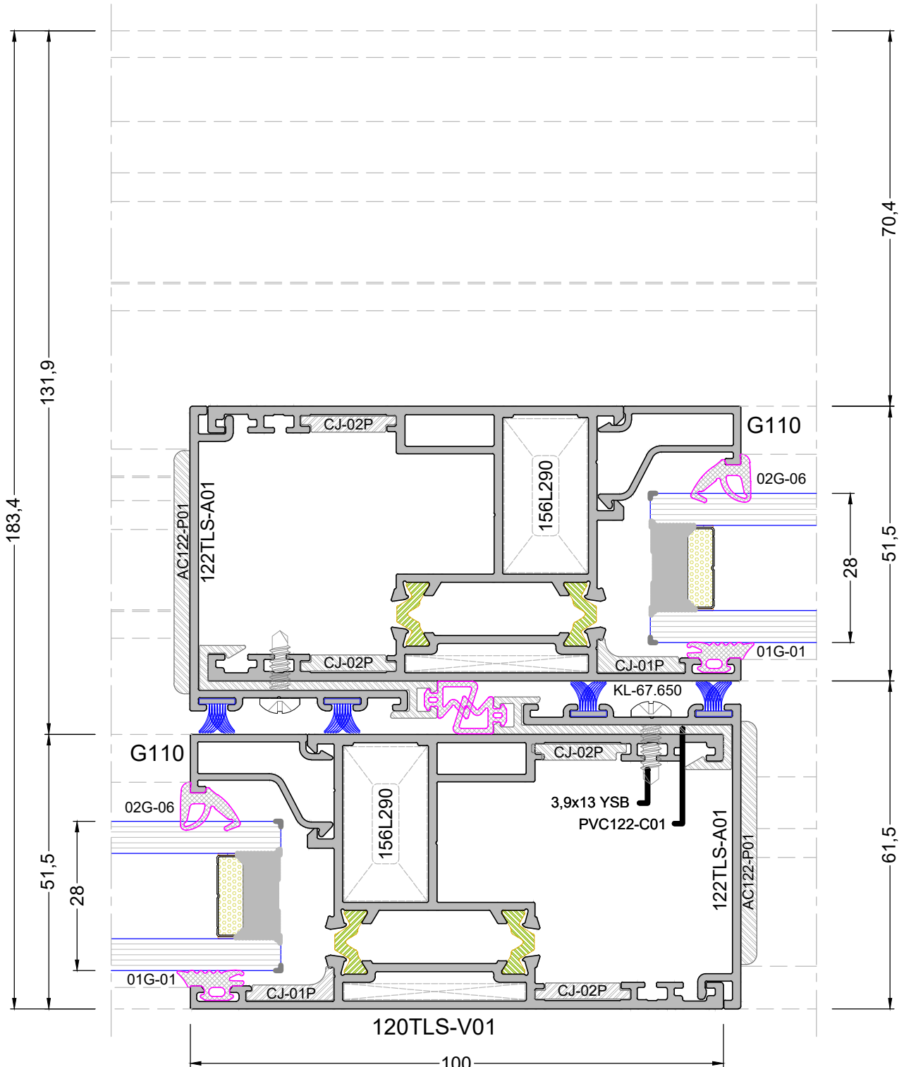
DETAY 3-9 DETAIL 3-9
