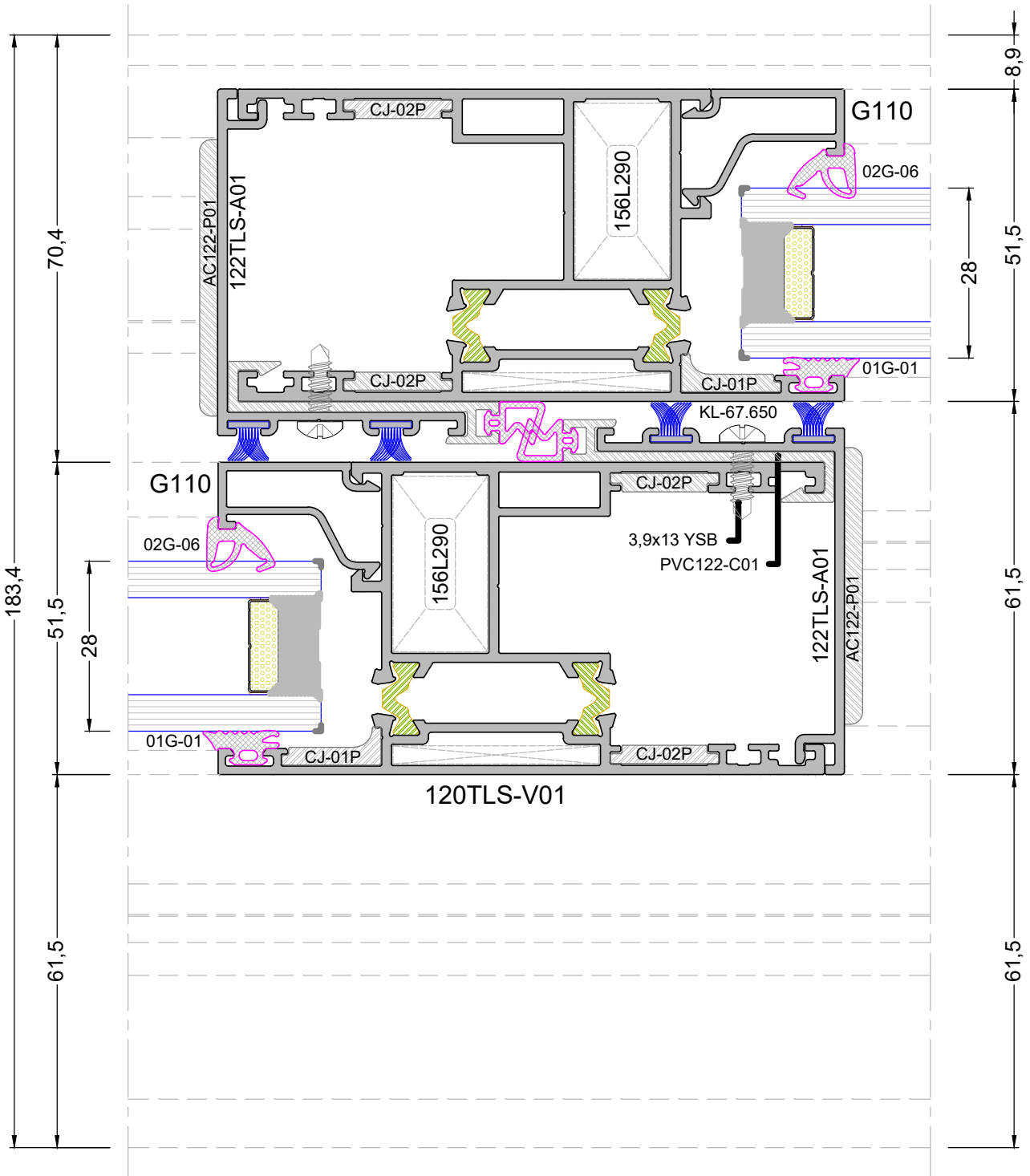
DETAY 3-10 DETAIL 3-10
