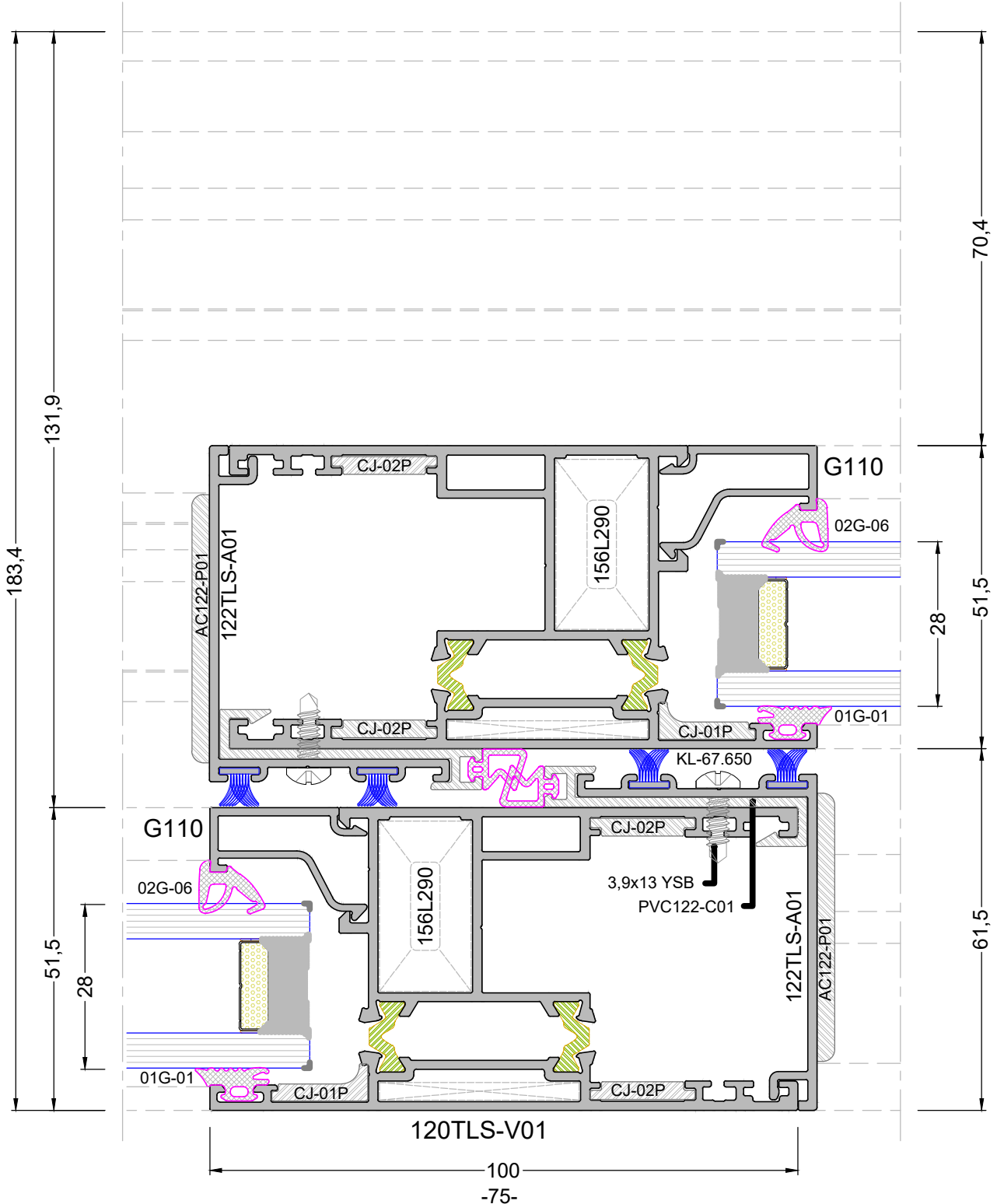
DETAY 3-2 DETAIL 3-2
