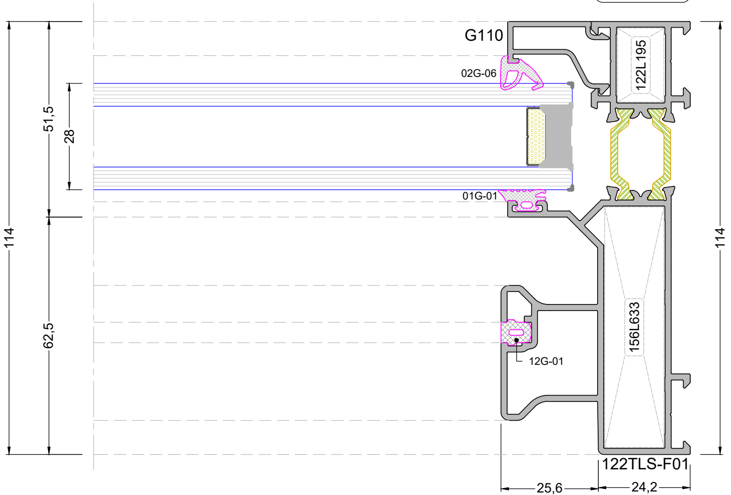
DETAY 1-17 DETAIL 1-17
