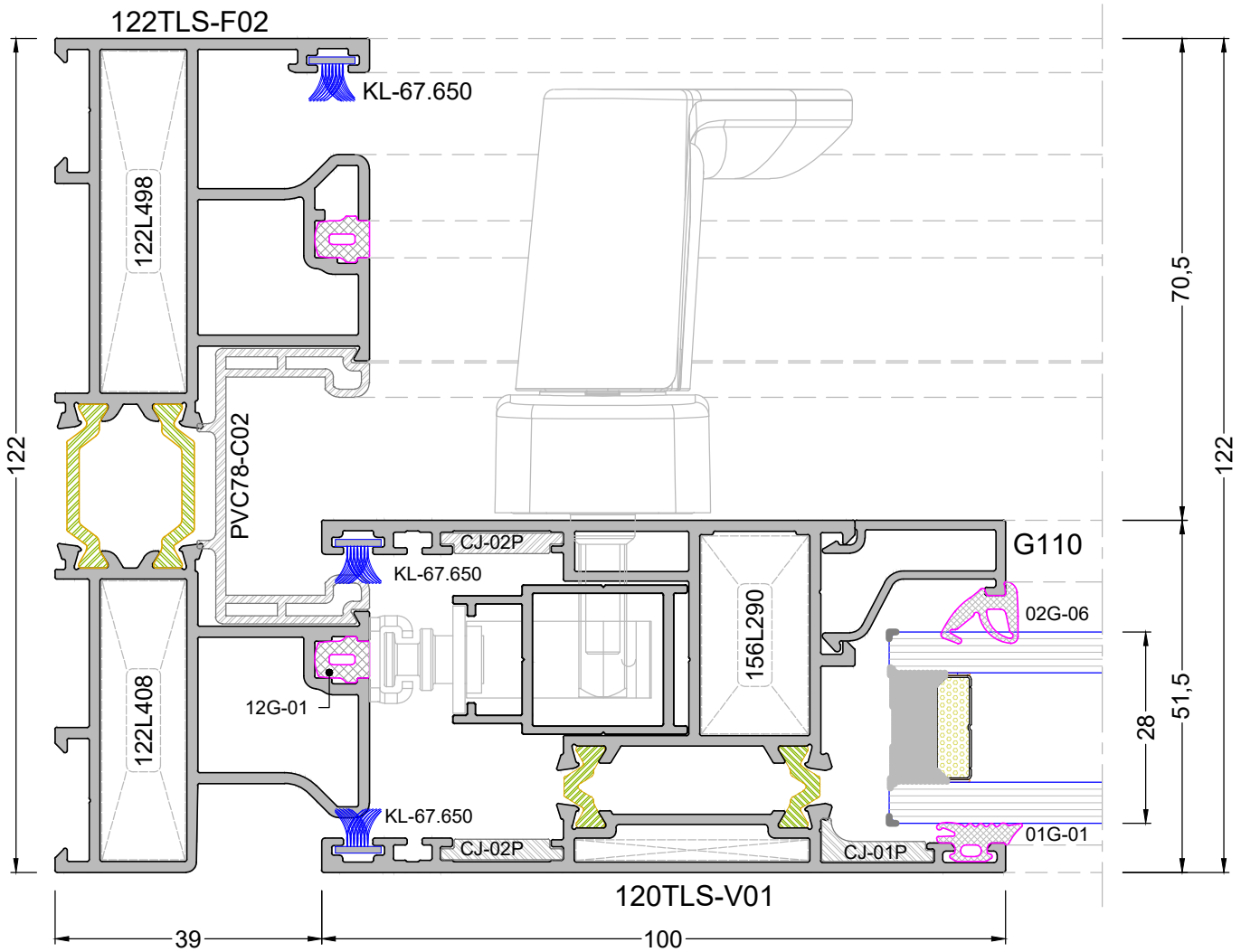
DETAY 2-14 DETAIL 2-14
