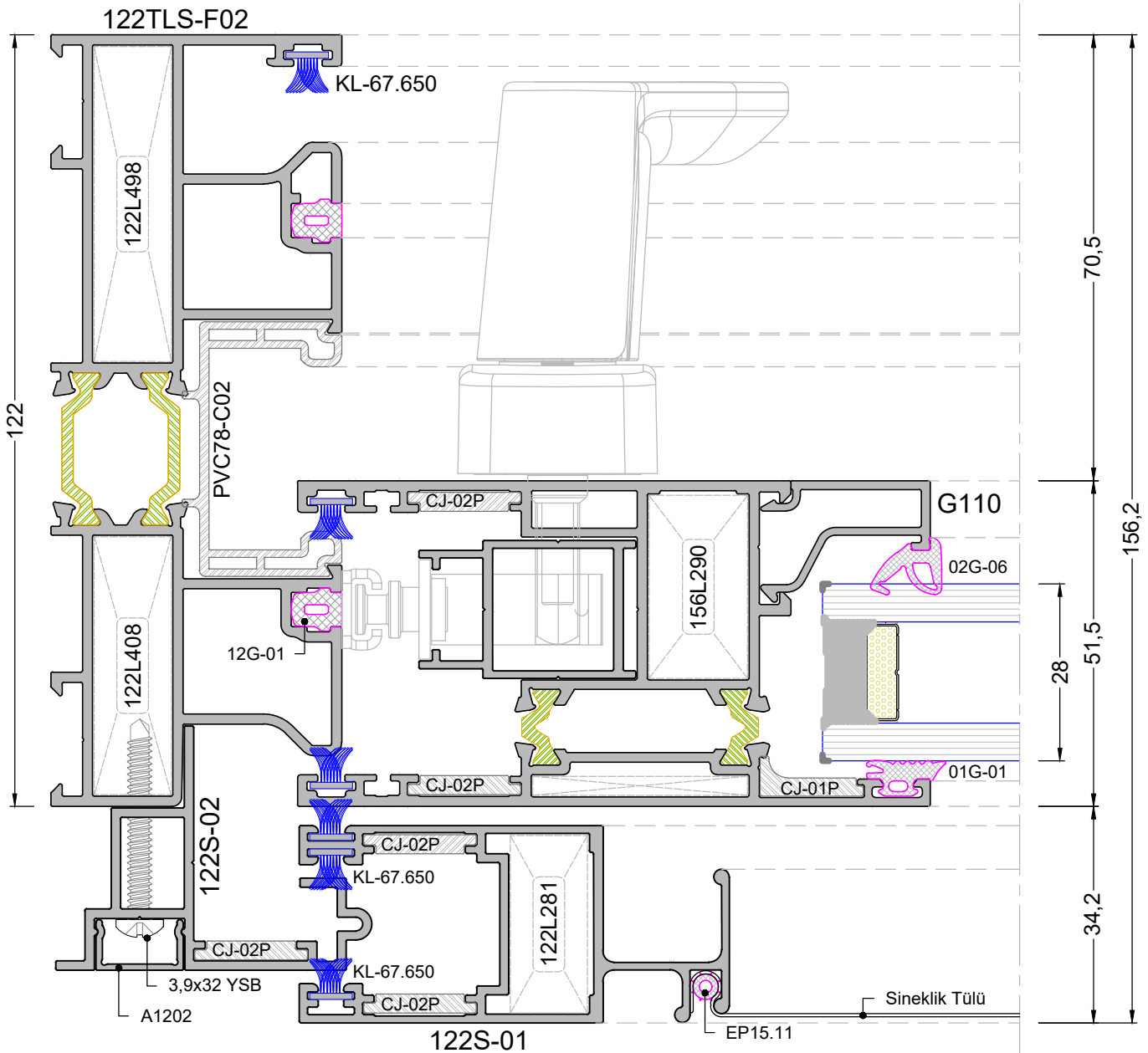
DETAY 2-22 DETAIL 2-22
