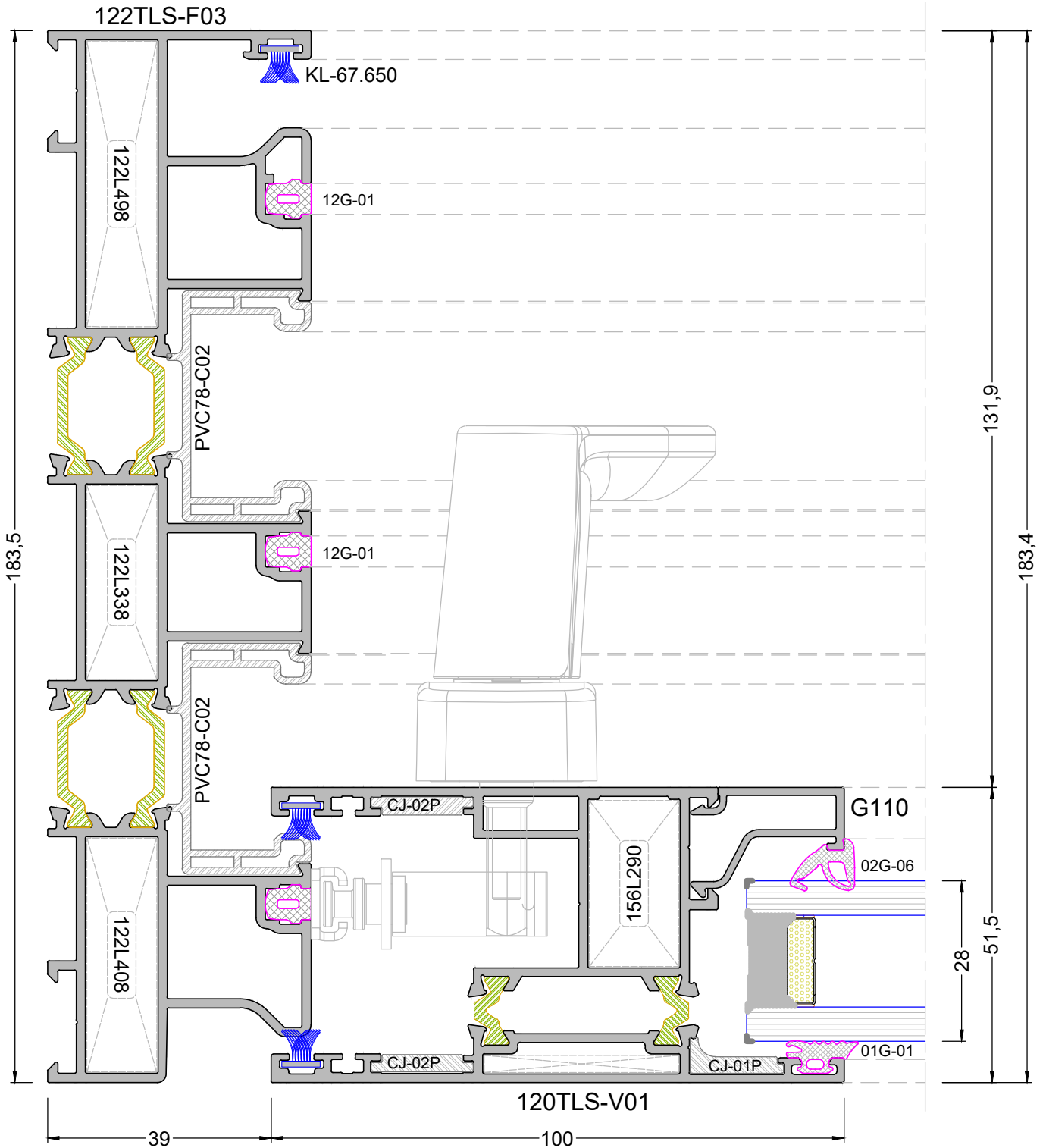
DETAY 3-8 DETAIL 3-8
