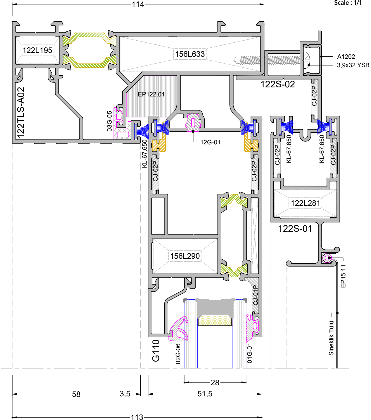
DETAY 1-28 DETAIL 1-28
