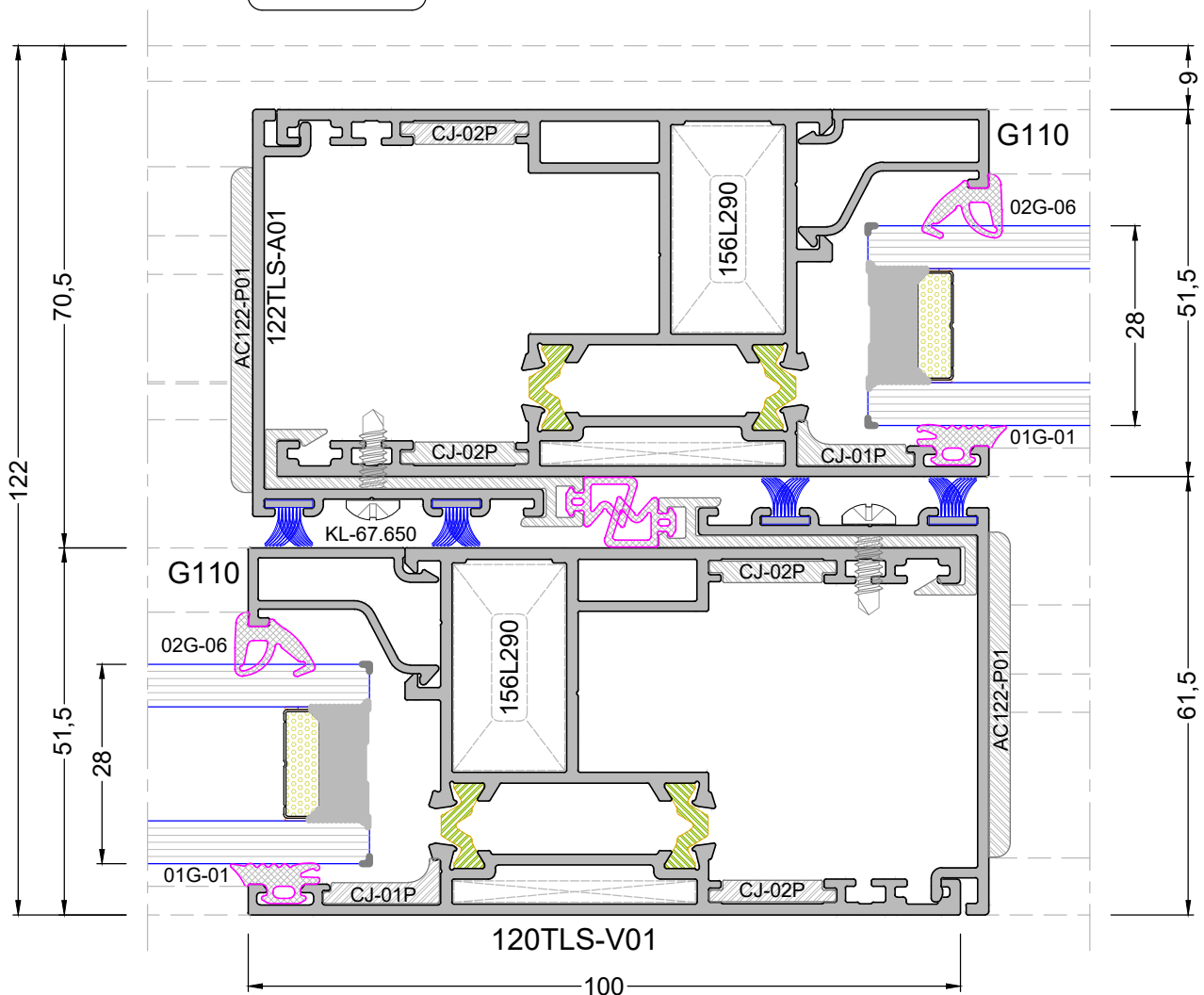
DETAY 2-2 DETAIL 2-2
