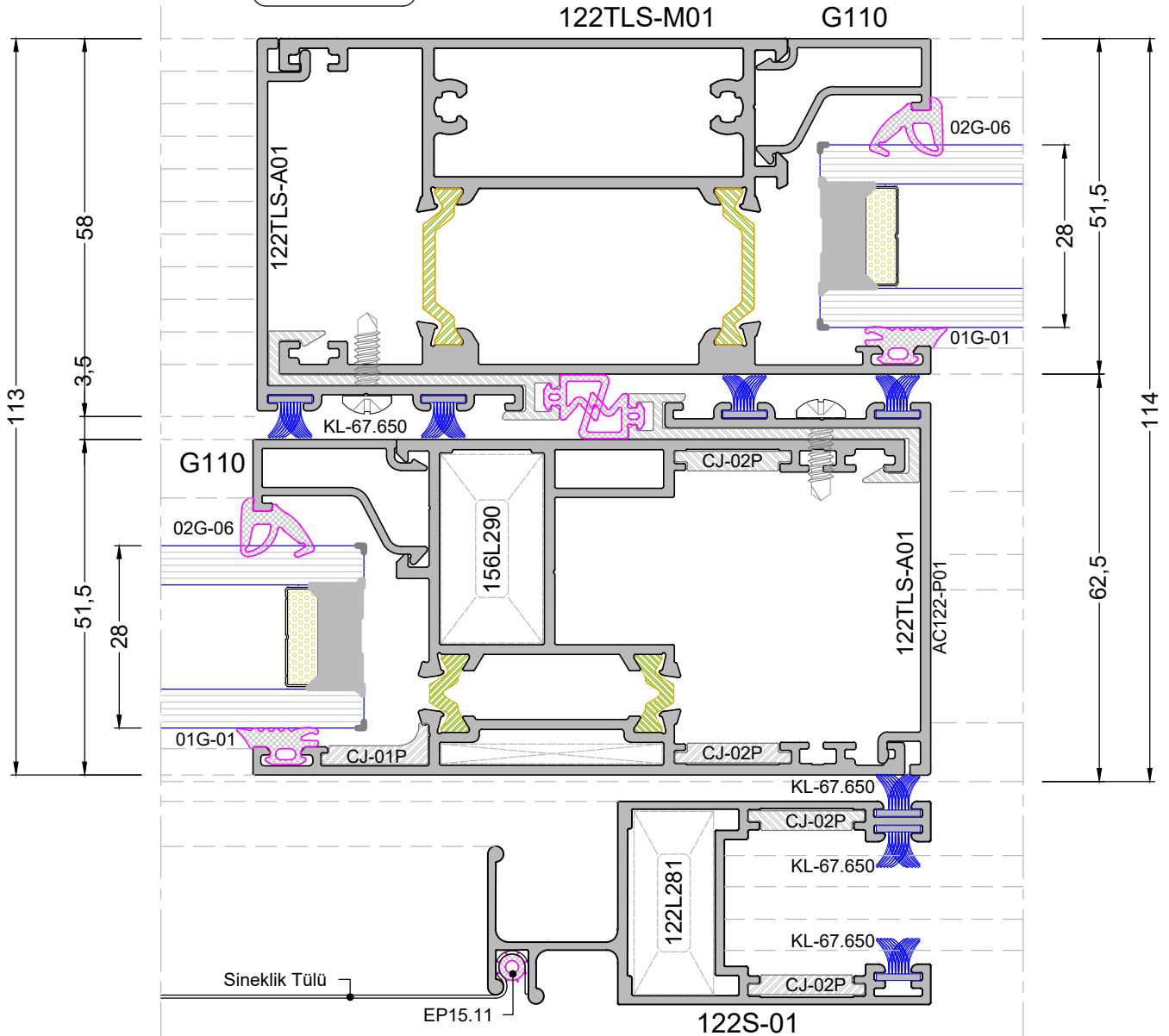
DETAY 1-11 DETAIL 1-11
