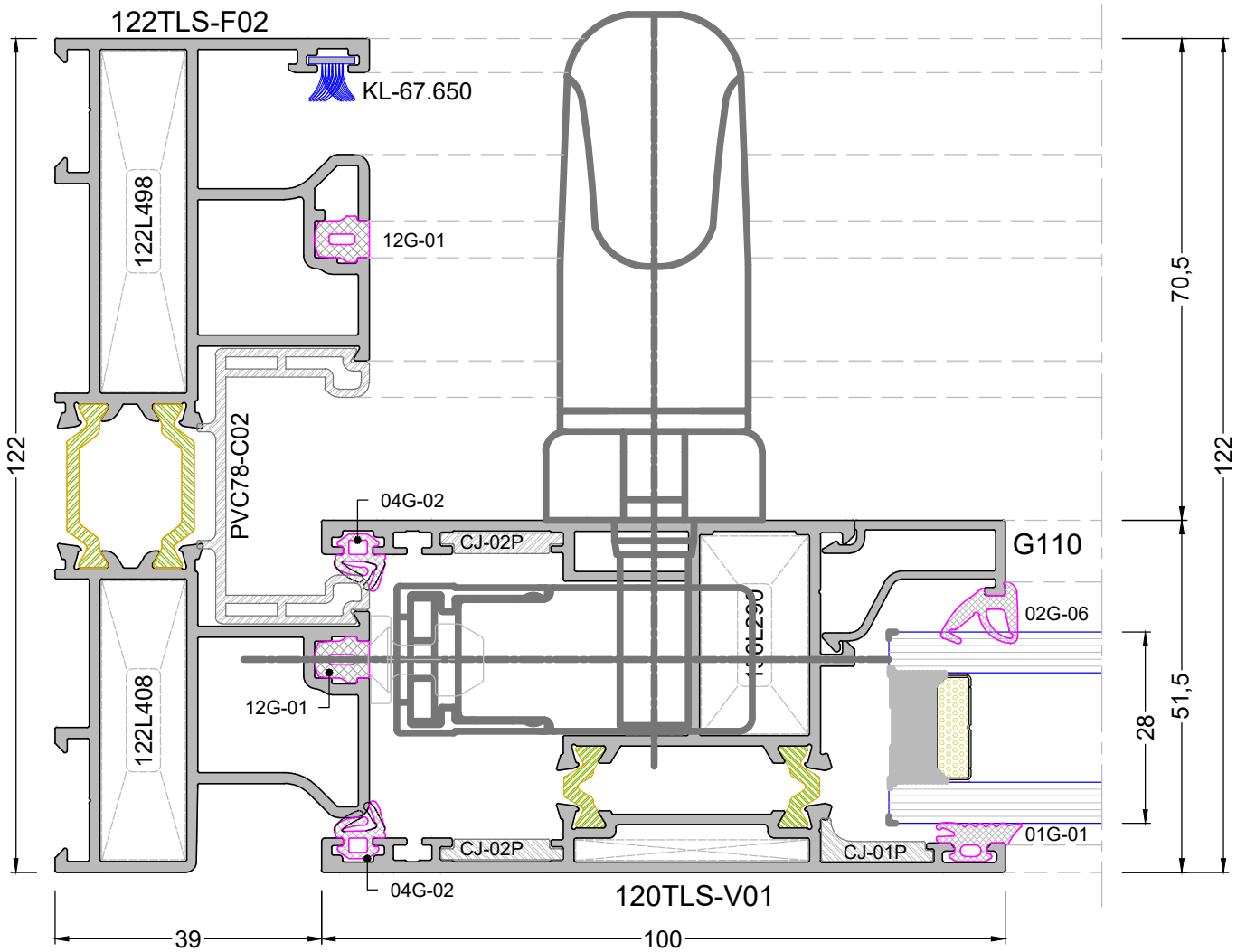
DETAY 2-1 DETAIL 2-1
