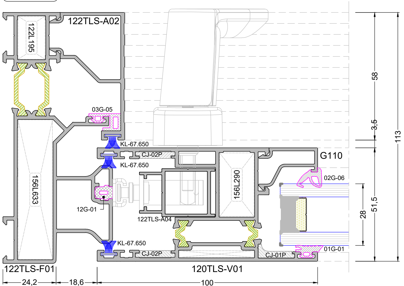
DETAY 1-15 DETAIL 1-15
