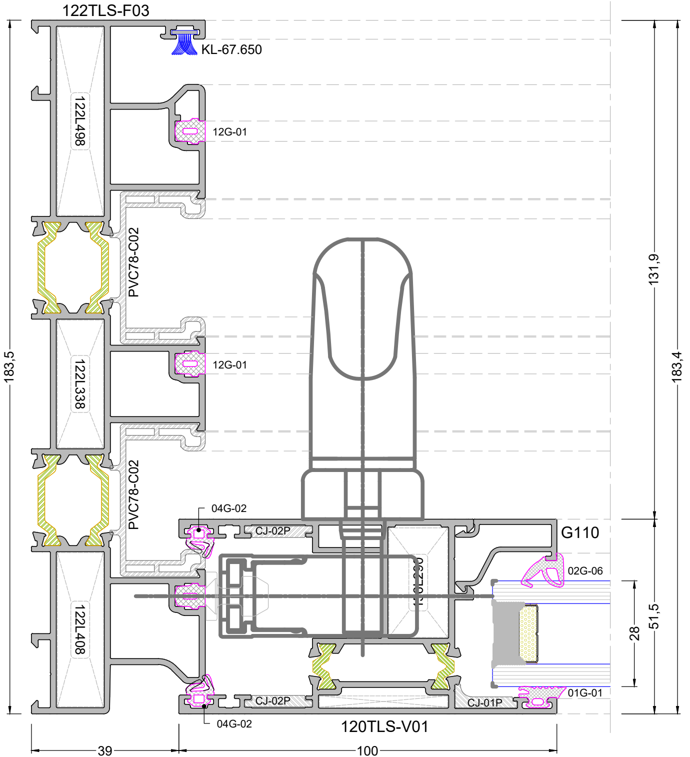
DETAY 3-1 DETAIL 3-1
