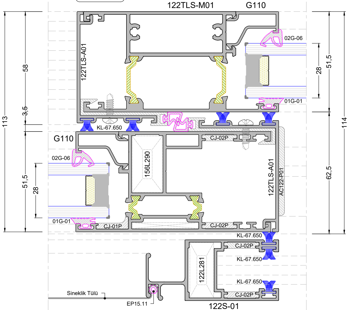
DETAY 1-25 DETAIL 1-25
