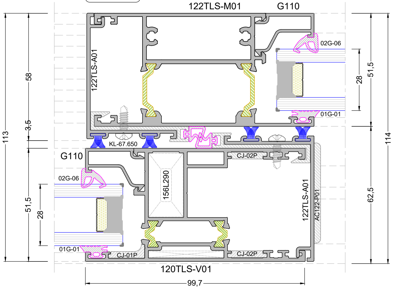
DETAY 1-16 DETAIL 1-16
