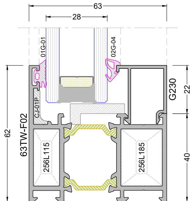
DETAY - 9 DETAIL - 9
