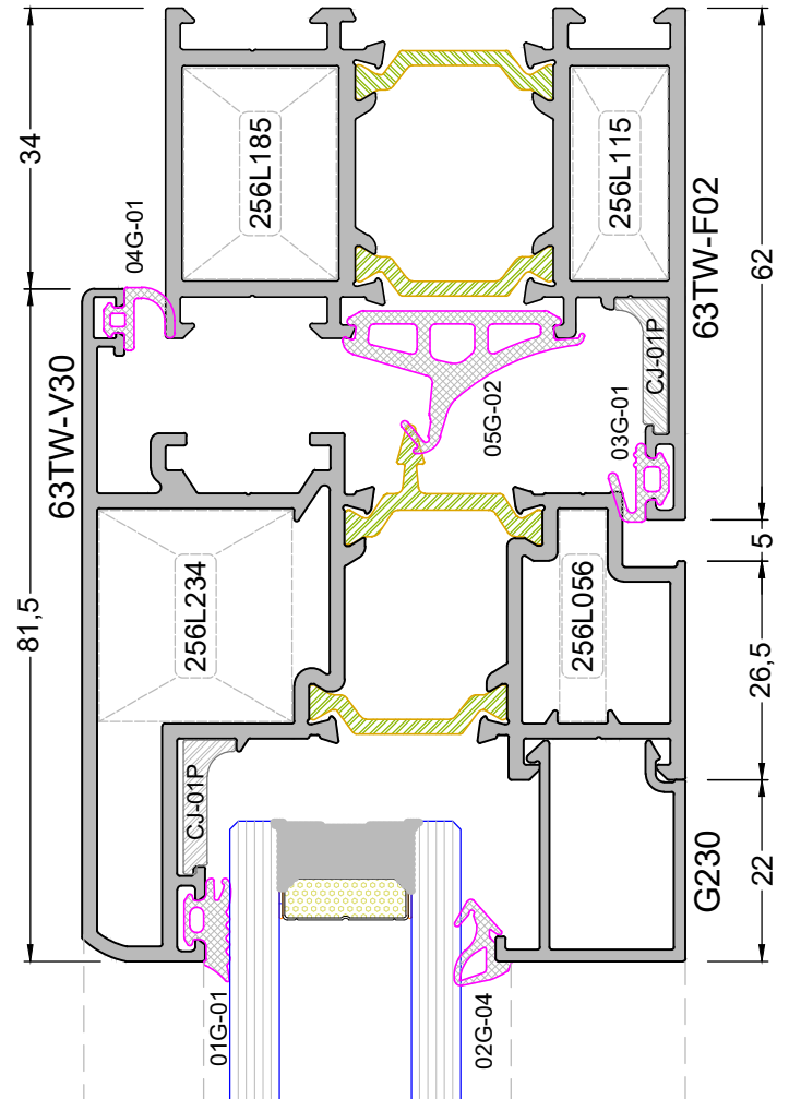
DETAY - 4 DETAIL - 4
