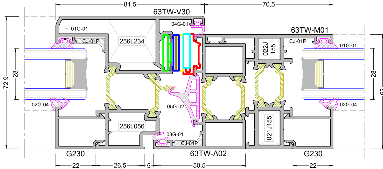
DETAY - 6 DETAIL - 6
