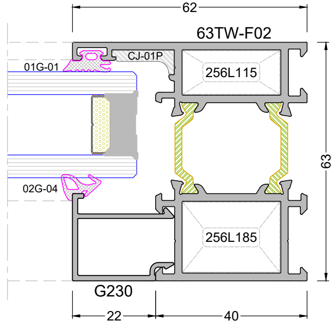
DETAY - 7 DETAIL - 7
