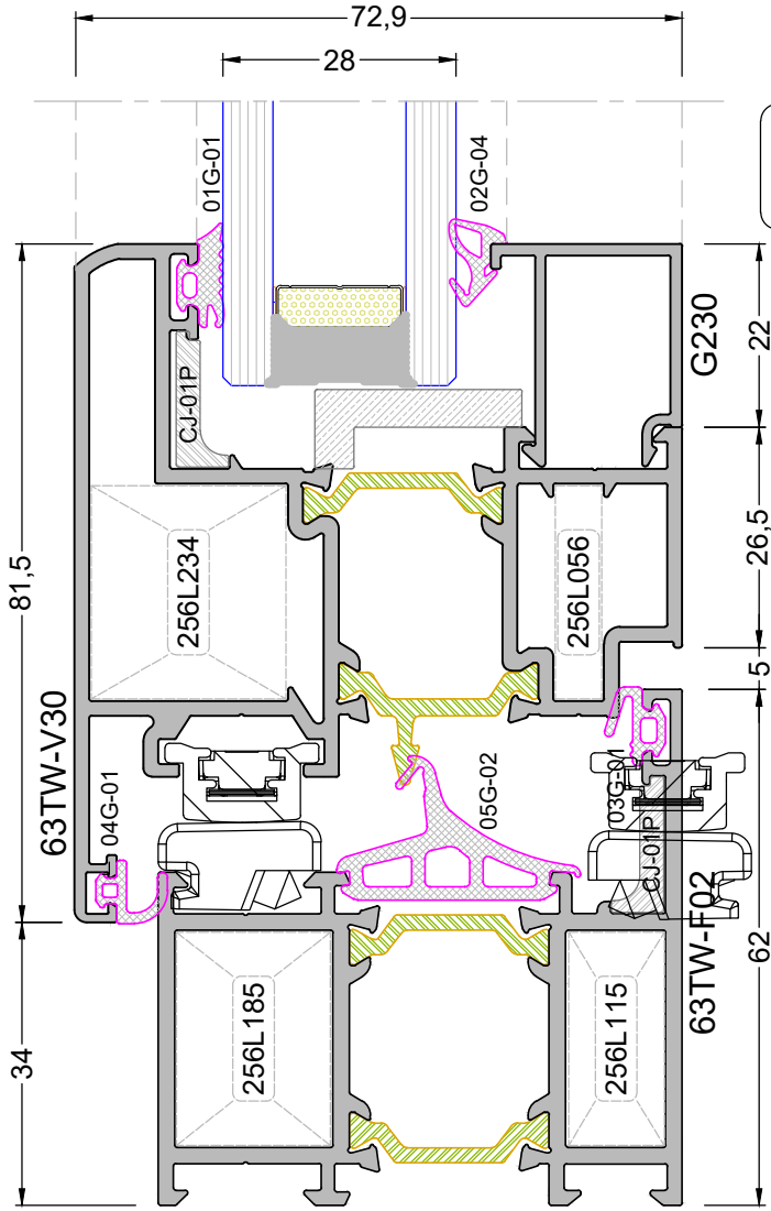
DETAY - 3 DETAIL - 3
