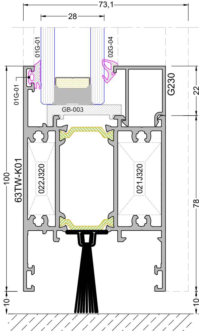
DETAY -13 DETAIL - 13
