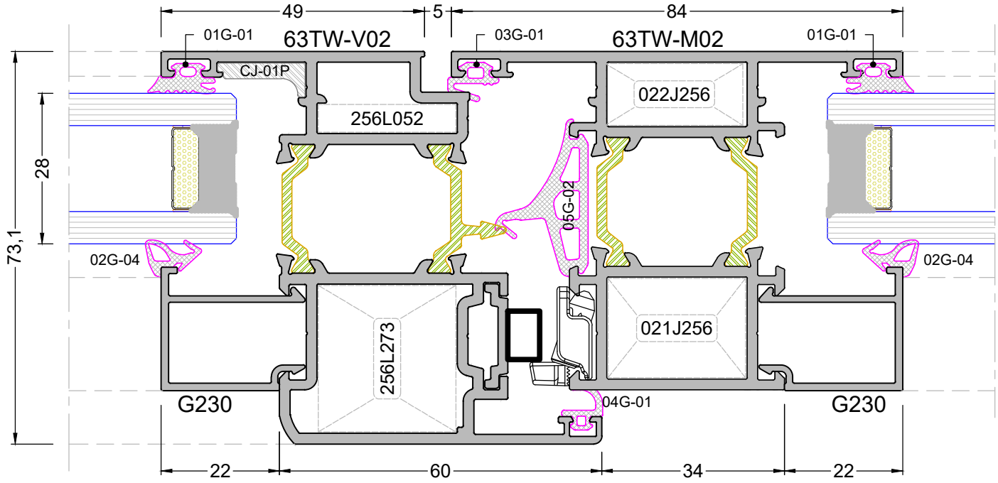
DETAY - 2 DETAIL - 2
