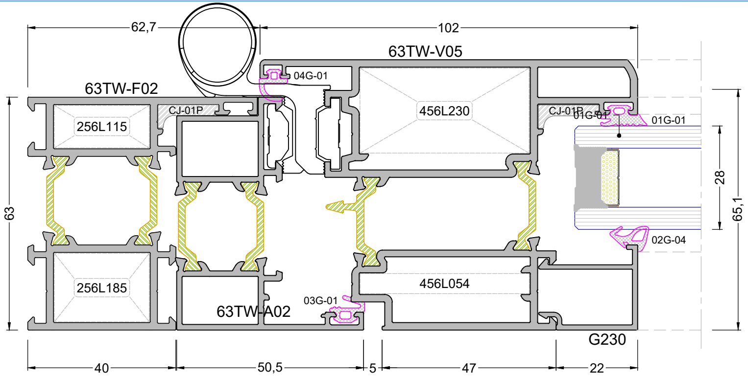
DETAY -14 DETAIL - 14
