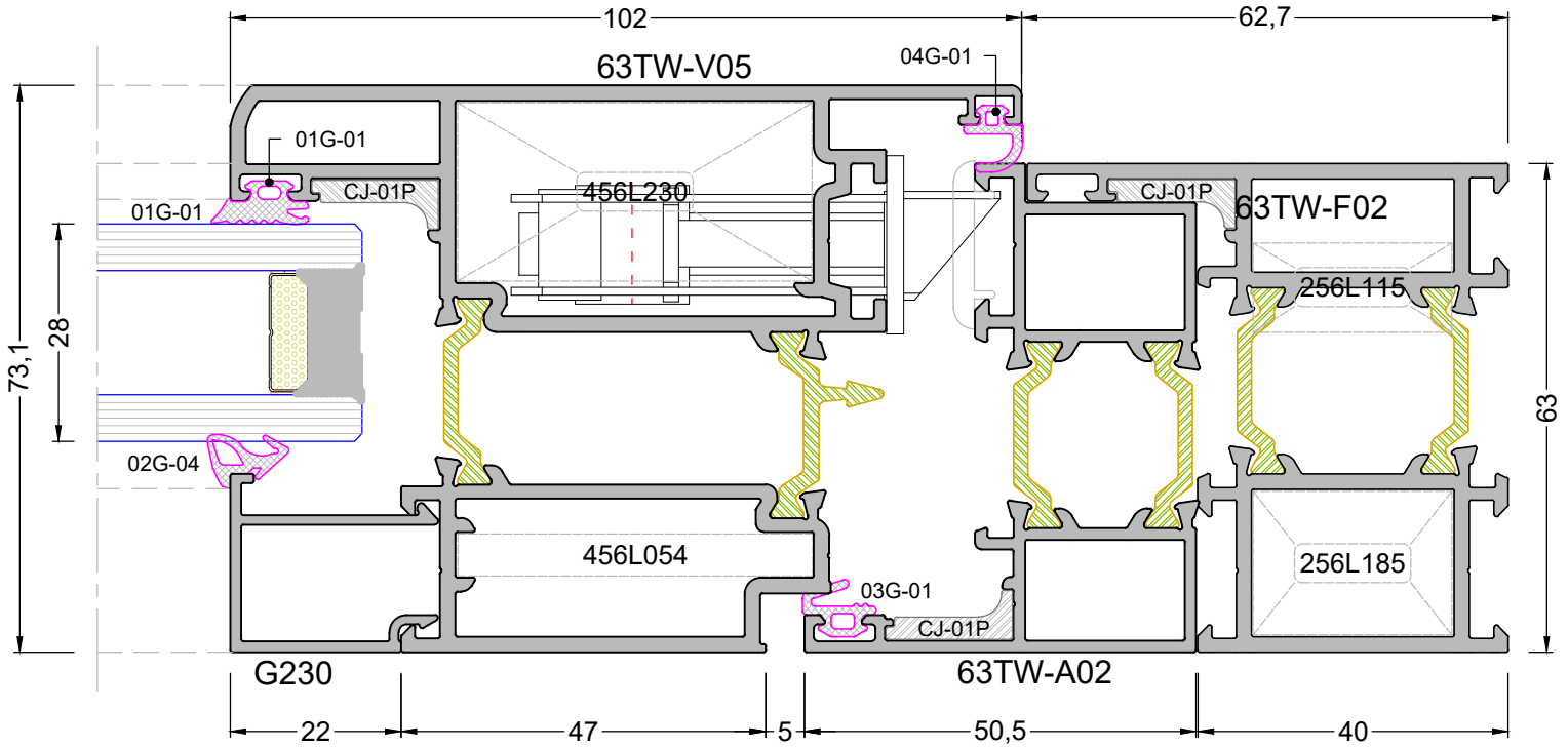
DETAY - 17 DETAIL - 17
