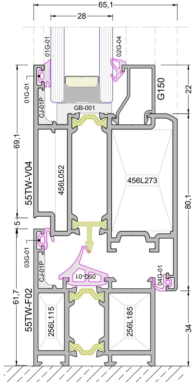
DETAY -13a DETAIL - 13a
