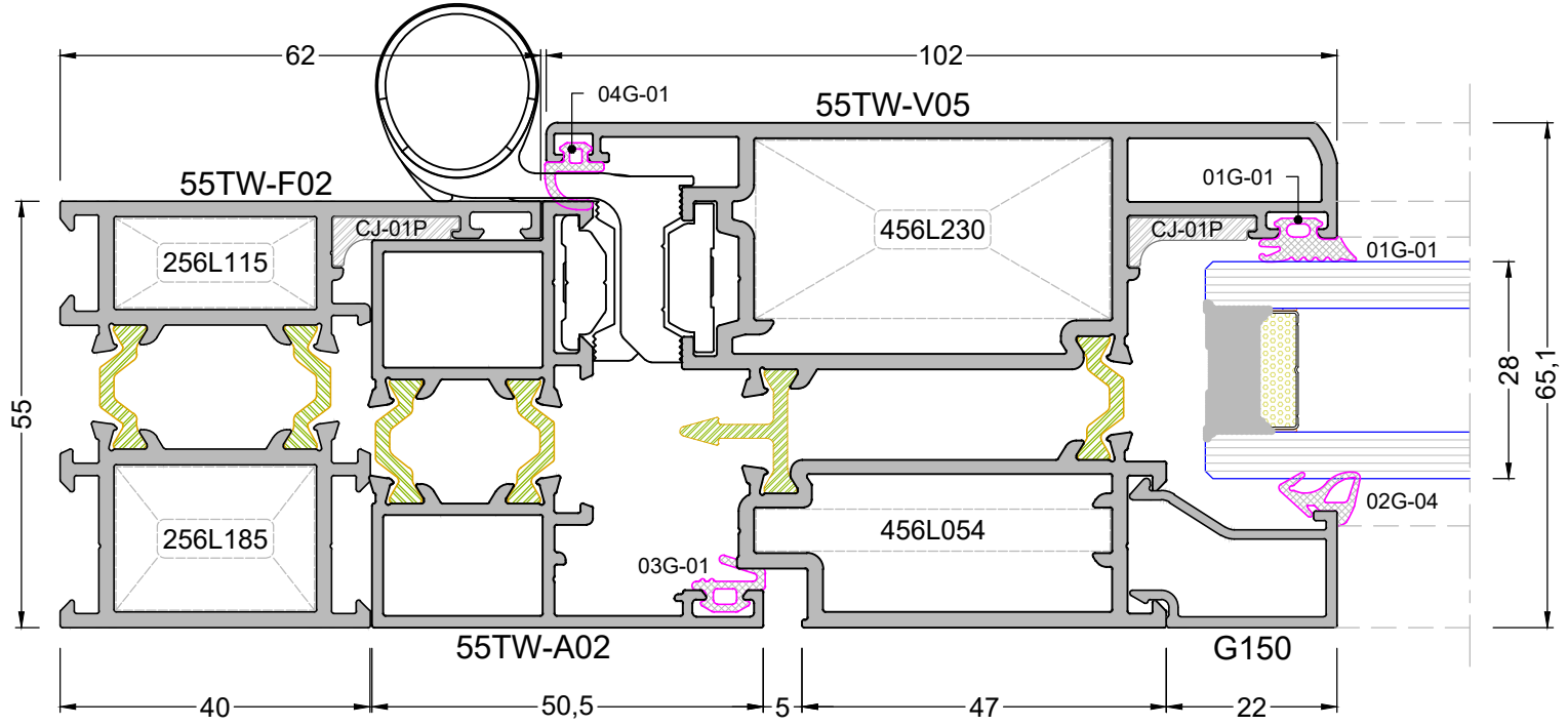
DETAY -14 DETAIL - 14
