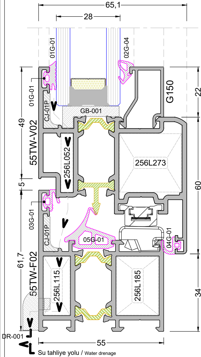
DETAY - 3 DETAIL - 3
