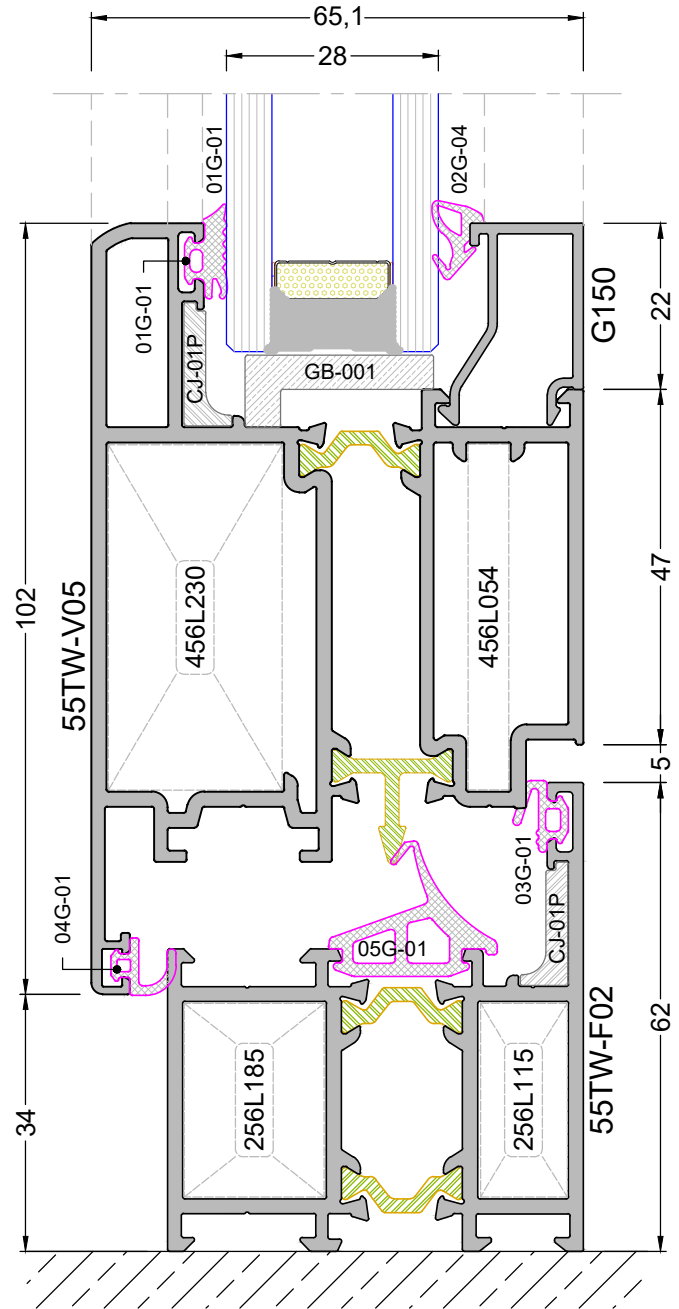
DETAY -16a DETAIL - 16a
