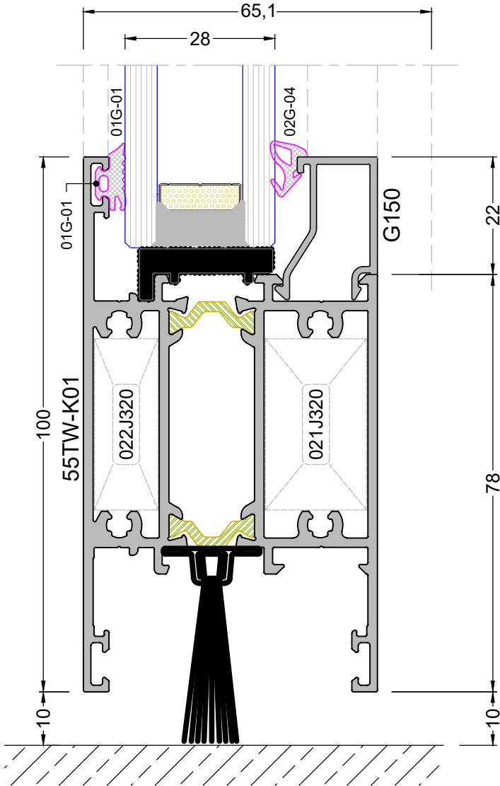
DETAY -16 DETAIL - 16
