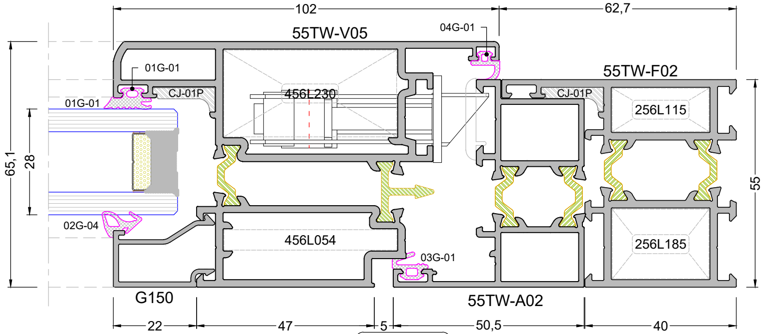
DETAY -17b DETAIL - 17b
