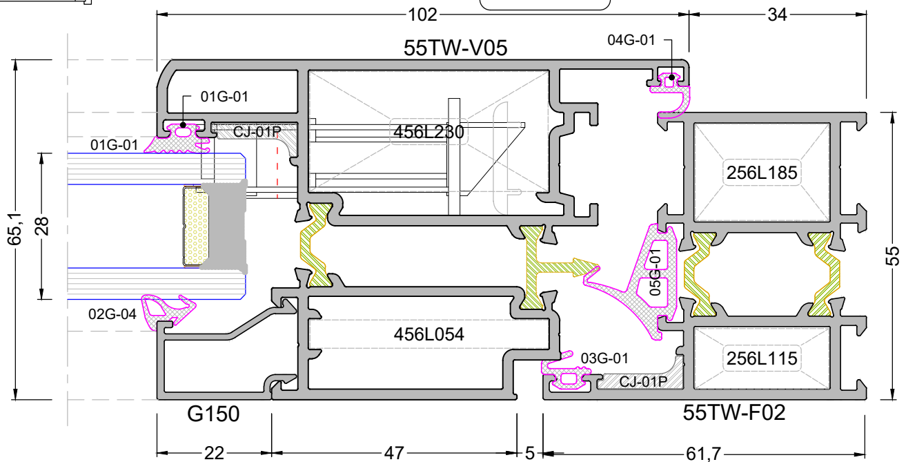
DETAY -17c DETAIL - 17c
