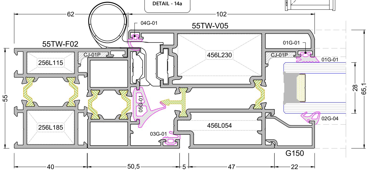
DETAY -14a DETAIL - 14a
