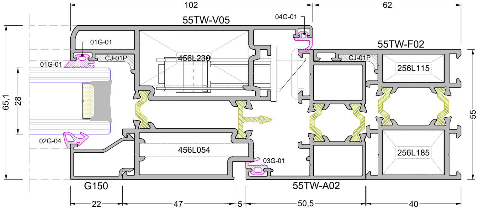
DETAY - 17 DETAIL - 17
