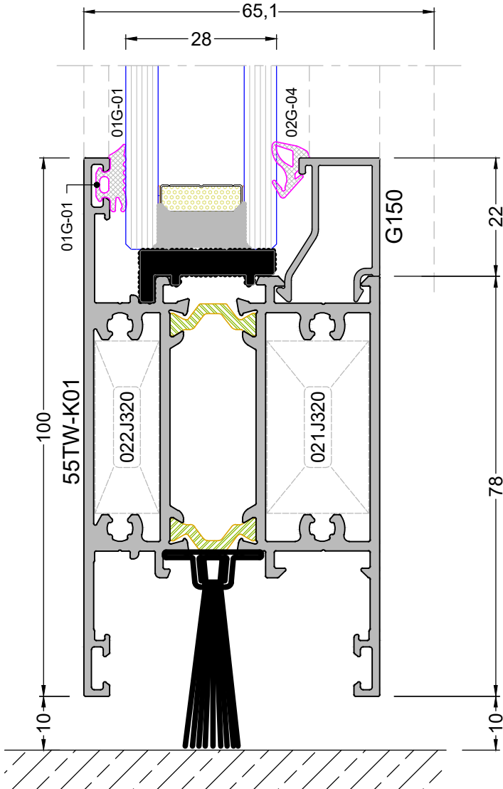
DETAY -13 DETAIL - 13
