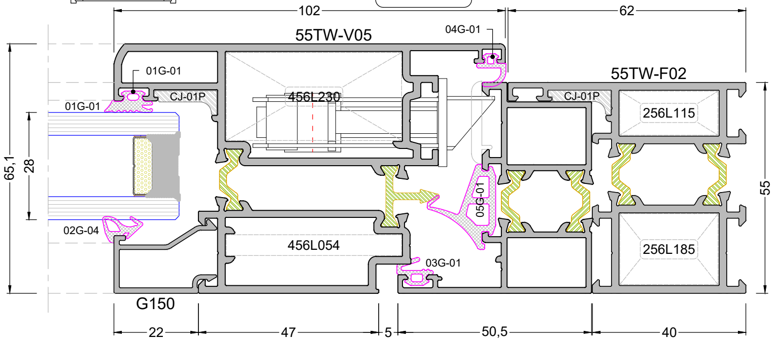
DETAY - 17a DETAIL - 17a
