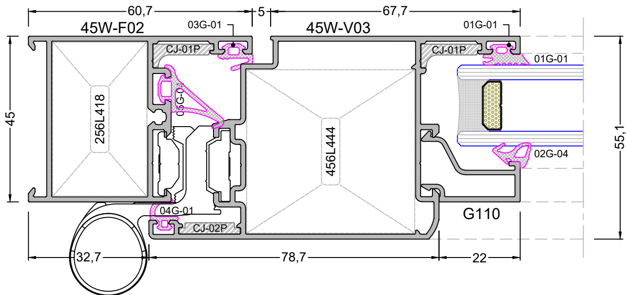
DETAY - 11a DETAIL - 11a
