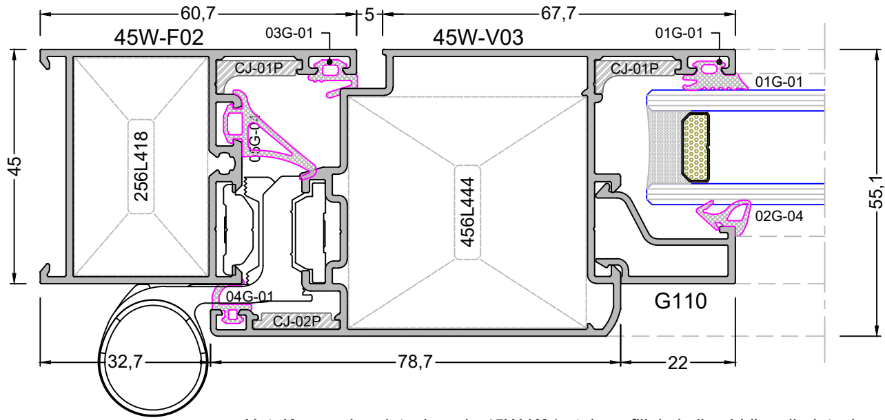
DETAY - 11 DETAIL - 11
