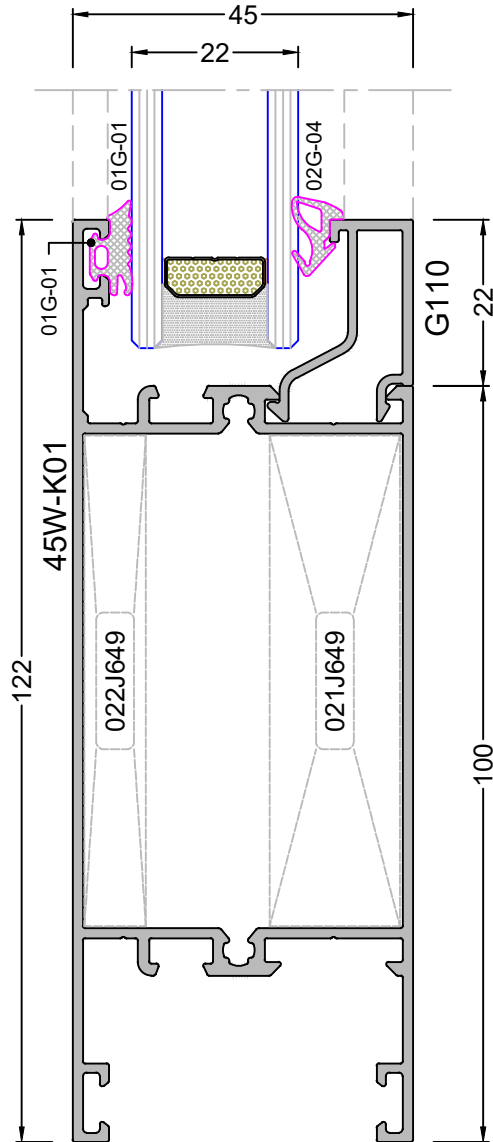
DETAY - 10 DETAIL - 10
