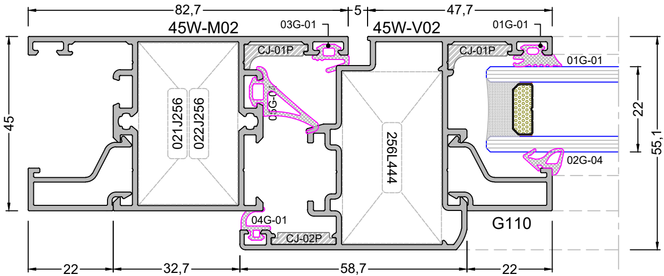
DETAY - 5a DETAIL - 5a
