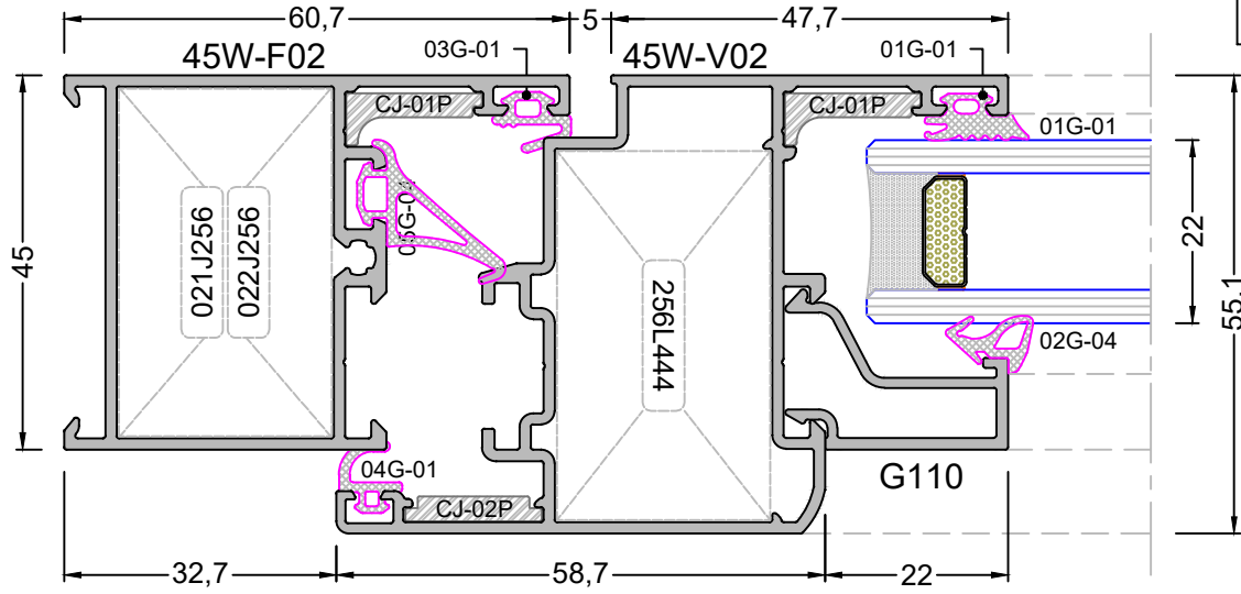
DETAY - 5 DETAIL - 5
