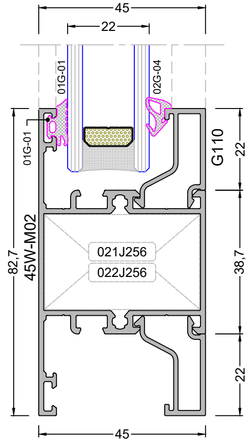
DETAY - 10a DETAIL - 10a
