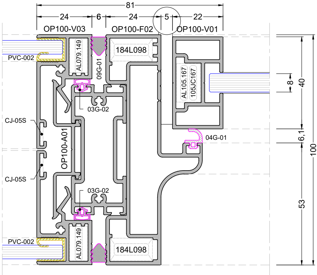
DETAY - 3 DETAIL - 3
