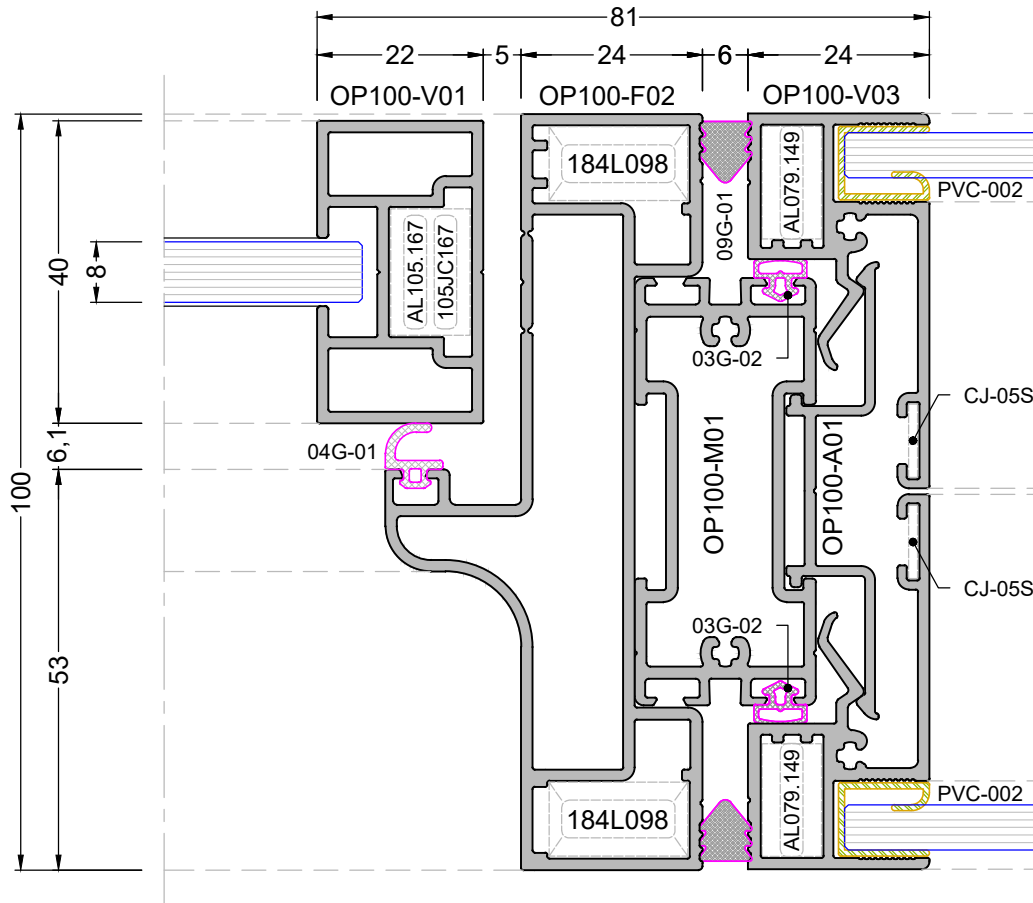
DETAY - 4 DETAIL - 4
